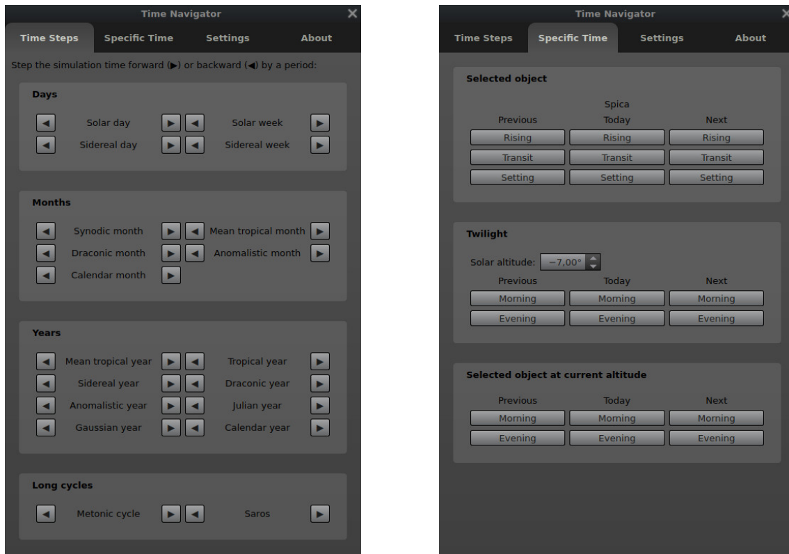
Figure 13.4: Interface of Time Navigator plugin: Time Steps tab (left) and Specific Time tab (right)
