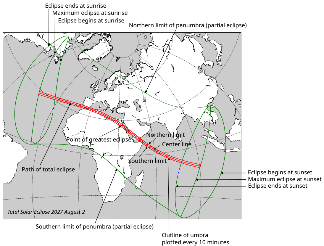
Figure 4.44: Key to solar eclipse map
