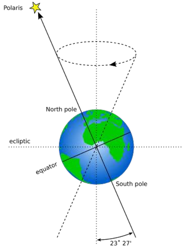
Figure 18.5: Precession
