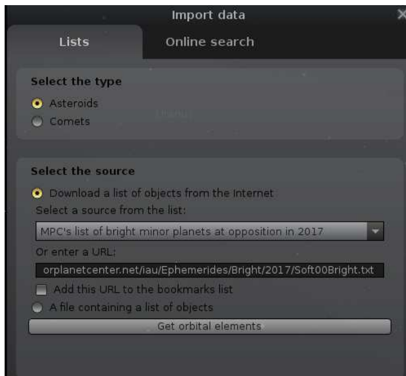
Figure 13.11: Interface of Solar System Editor plugin: Import data dialog
