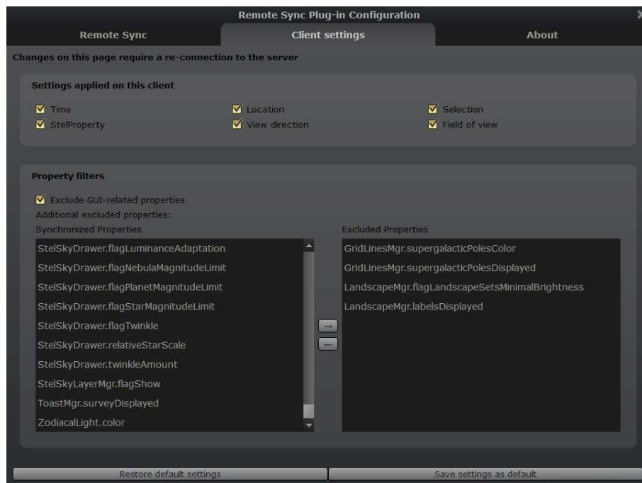
Figure 13.8: RemoteSync client settings window
